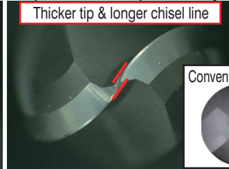
③ Optimized Ball Tip Geometry
