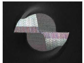
End mill for steels (2 flutes) \phi 1 \times \text{L2.5}
