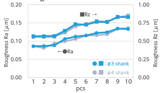
Roughness of concave surface
