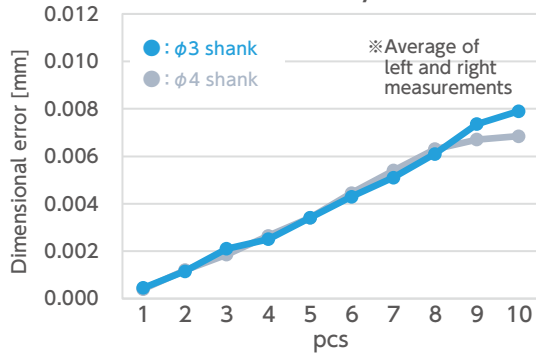
Dimensional accuracy of vertical wall
