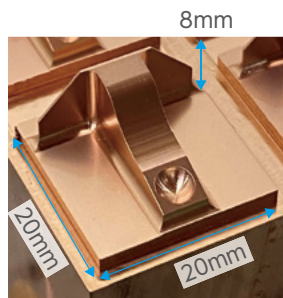
Milling shape
